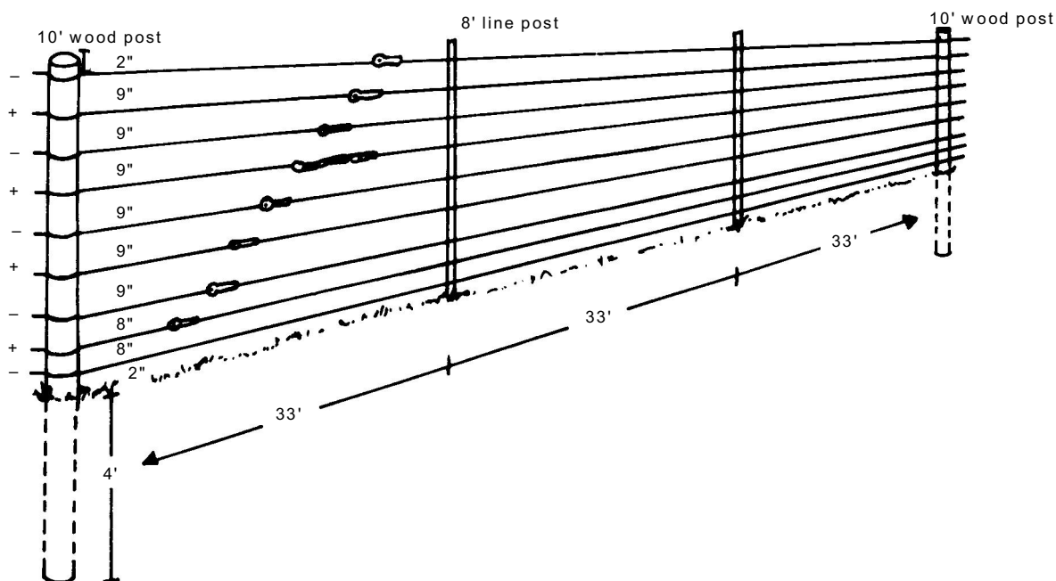
Figure 3. The nine-wire vertical deer fence. Note: the seven-wire fence described in previous editions of this bulletin has been expanded to nine wires to prevent reported deer penetration of the previous 12" spacing. The low 2" wire (strung very tightly) prevents deer from squeezing under the fence.
