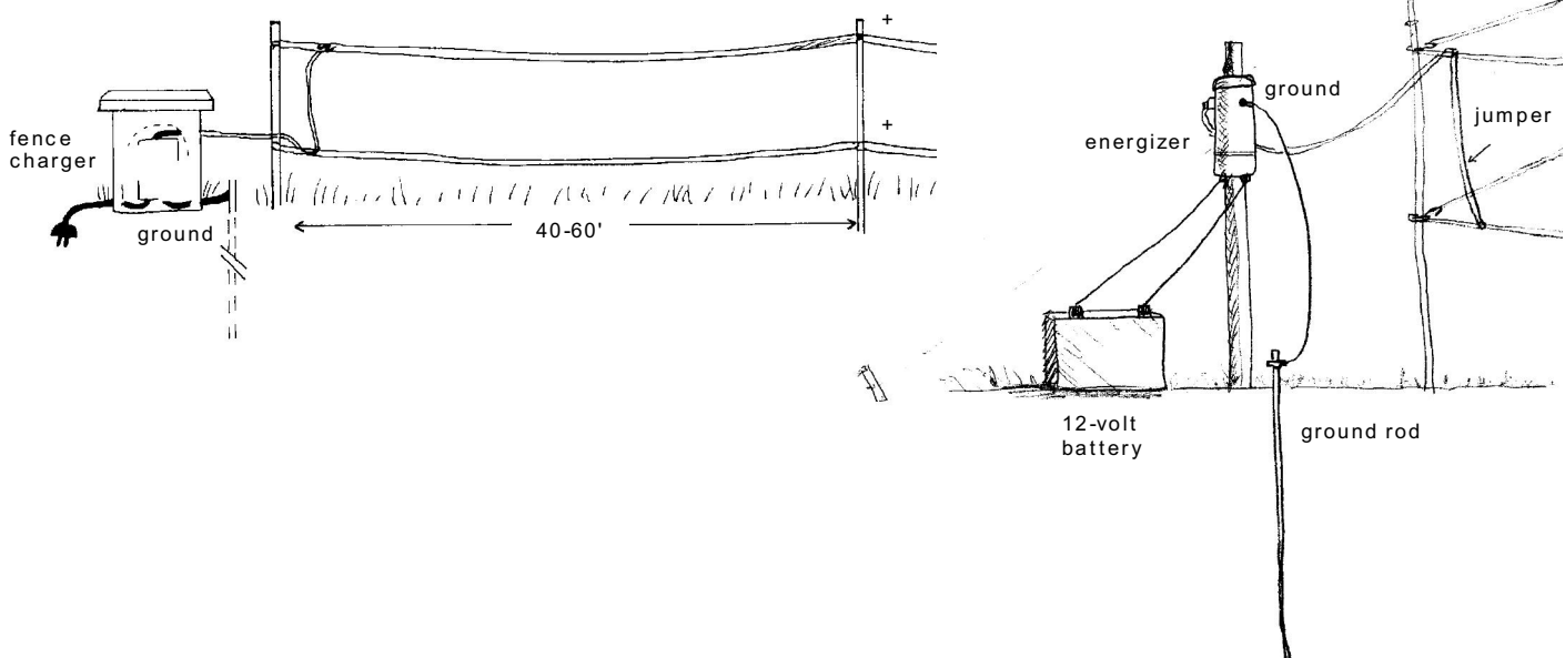
Figure 2. The polytape fence.
